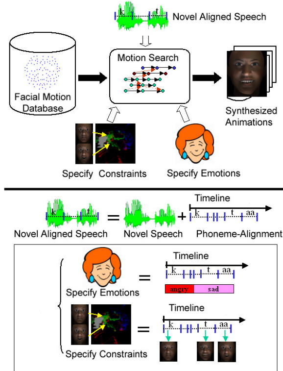
Figure 1: Illustration of the eFASE pipeline. At the top, given novel phoneme-aligned speech and specified constraints, this system searches for best-matched motion nodes in the facial motion database and synthesizes expressive facial animation. The bottom illustrates how users specify motion-node constraints and emotions with respect to the speech timeline.
