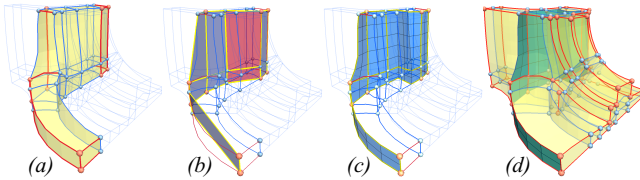
Figure 9: (a) A candidate in a Fandisk hex-mesh; (b) the computed patch configurations, which are indicated by colored planes (blue for original configurations and red for diagonal configurations); (c) the extracted quad surface; and (d) the reconstructed simplified base-complex.
