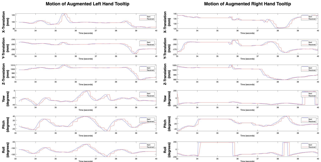
FIGURE 12 Graphical representation of delay in receiving information at the remote location for a time period of 7 s. The pose of augmented instrument tooltip M_{ToolTips}(t) for left M_{ToolTips[1]}(t) and right M_{ToolTips[2]}(t) hand is acquired at remote location workstation and send to operating room workstation. The operating room workstation receives the M_{ToolTips}(t) with a delay
