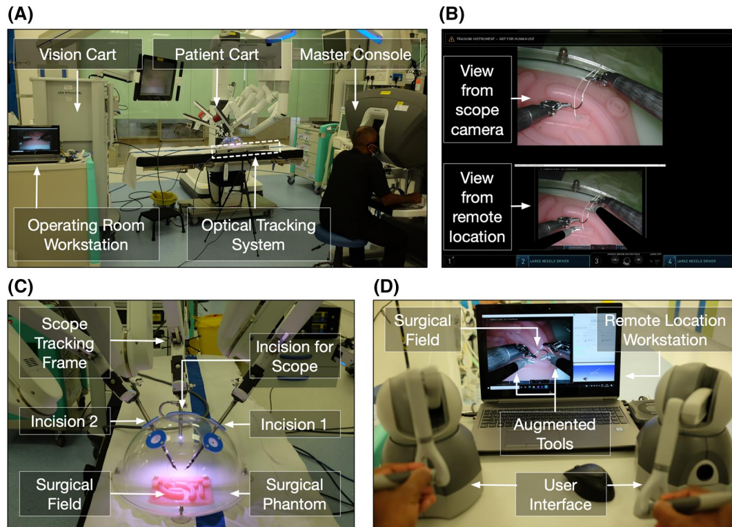
FIGURE 7 Tele-mentoring framework tested for a minimally invasive robotic surgical setup. (A) Setup of the tele-mentoring framework at the operation room; (B) View from the master console; (C) Surgical phantom used to mimic incisions and surgical field; (D) Setup of the tele-mentoring framework at the remote location
